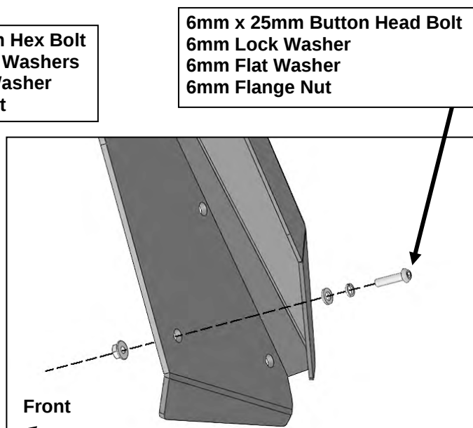
(Fig 6) Attach rear of Fender to hole in side of body
