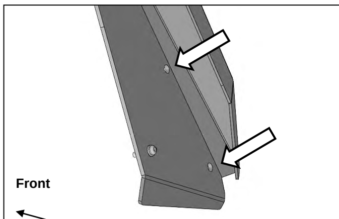
(Fig 7) To help identify the correct factory holes in body panel, place marks on holes before drilling
